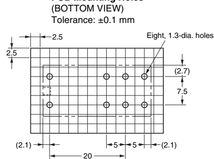
PCB Mounting Hole
