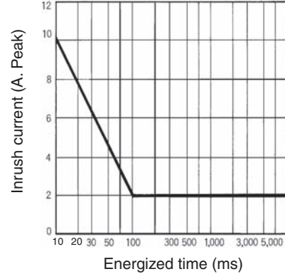
G3FD-102SN-VD/102S-VD
