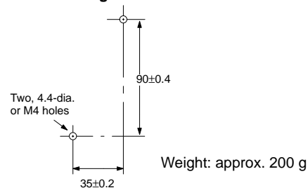
Mounting Holes
