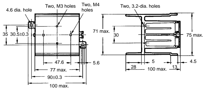
Mounting Holes
