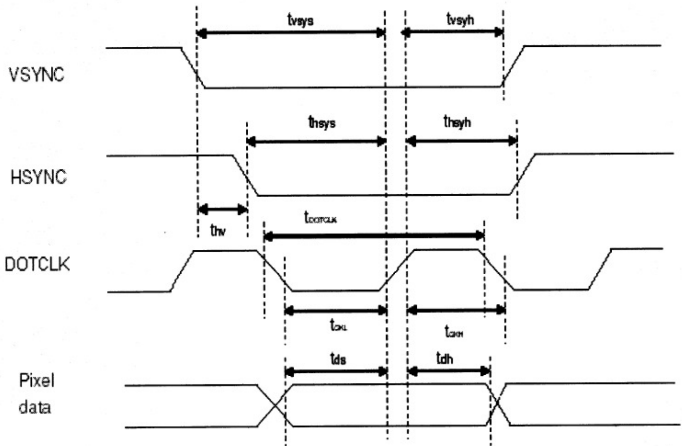
Pixel timing
