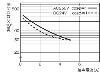
形H3YN-2/-21
