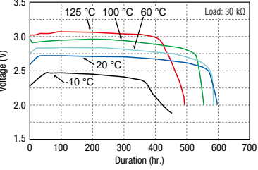
■ Discharge temperature characteristics (Example: BR1225A)
