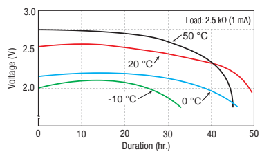
■ Discharge temperature characteristics (Example: BR435)
