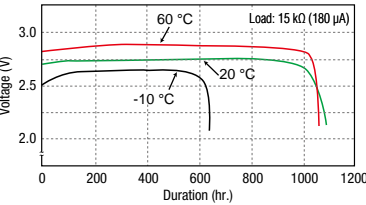
■ Discharge temperature characteristics (Example: BR2032)
