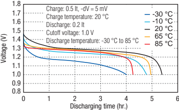
■ Example discharge characteristics
