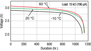
■ Discharge temperature characteristics (Example: CR2032)
