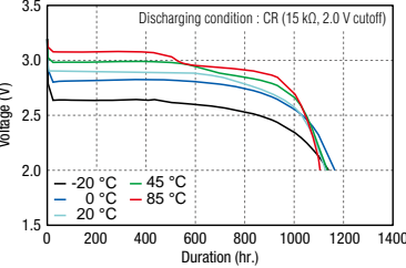
■ Discharge temperature characteristics (Example: CR2032A)
