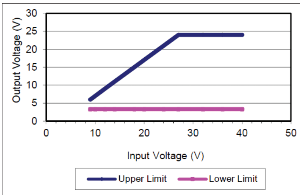
Output voltage vs input voltage operating range i6A Series
