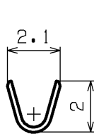
WIRE BARREL
