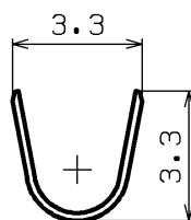
INSULATION BARREL
