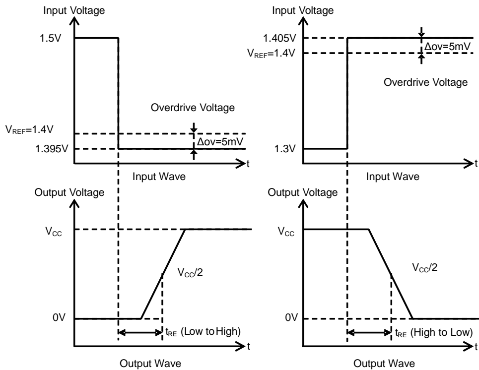
Figure 41. Response Time
