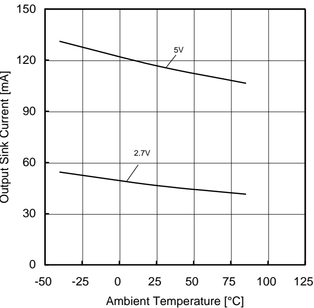
Figure 11. Output Sink Current vs Ambient Temperature (OUT=VDD)
