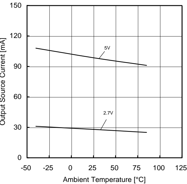
Figure 9. Output Source Current vs Ambient Temperature (OUT=0V)
