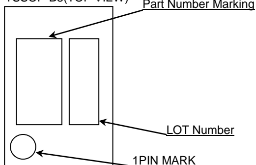
TSSOP-B8(TOP VIEW)
