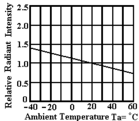
Radiant Intensity vs. Ambient Temperature
