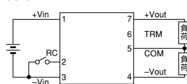
CC10-xxxxDx-E
