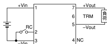
CC6-xxxxSx-E
