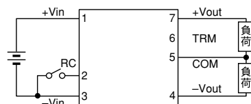
CC6-xxxxDx-E
