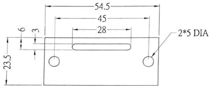
Gasket dimension
