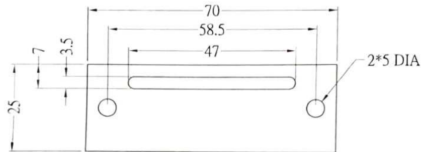
Gasket dimension
