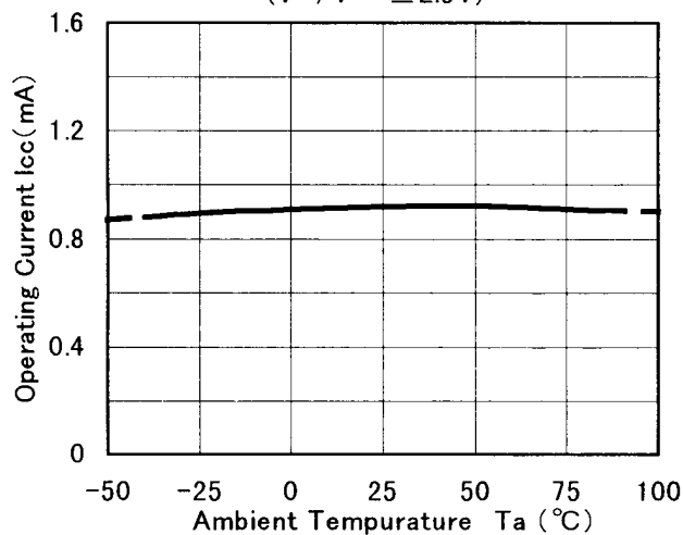
Operating Current vs. Temperature ( V^+/V^- = \pm 2.5V )
