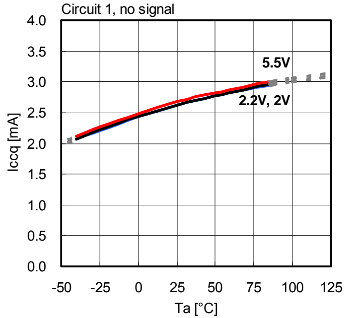
Operating Current I_{ccq} versus Ambient Temperature T_a
