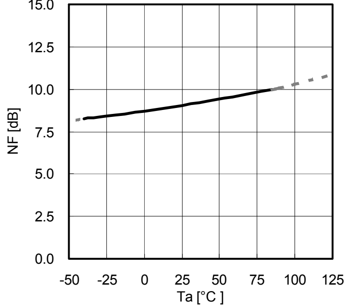
Noise Figure NF versus Ambient Temperature Ta
