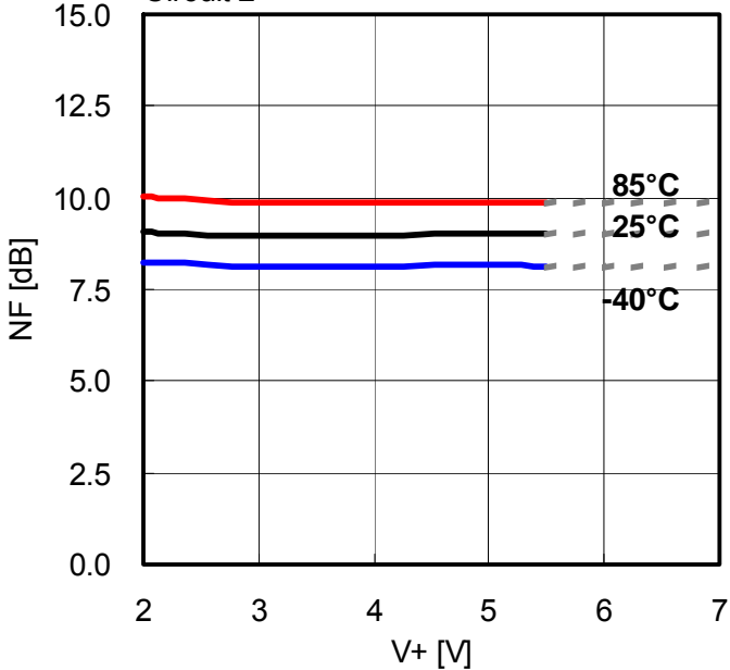
Noise Figure NF versus Supply Voltage V+
