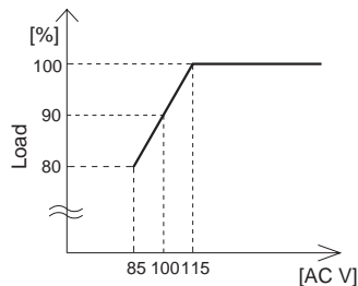
Fig.3.2 Input voltage derating curve
