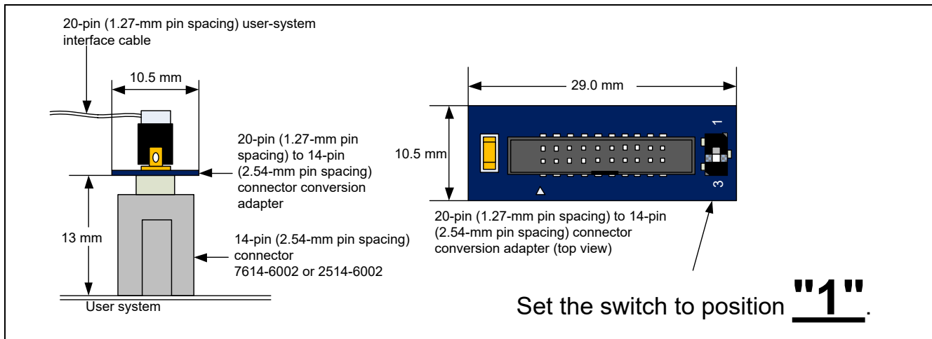
Figure 2.3 Connecting the User System Interface Cable to the 14-Pin Connector of the E2 Emulator
