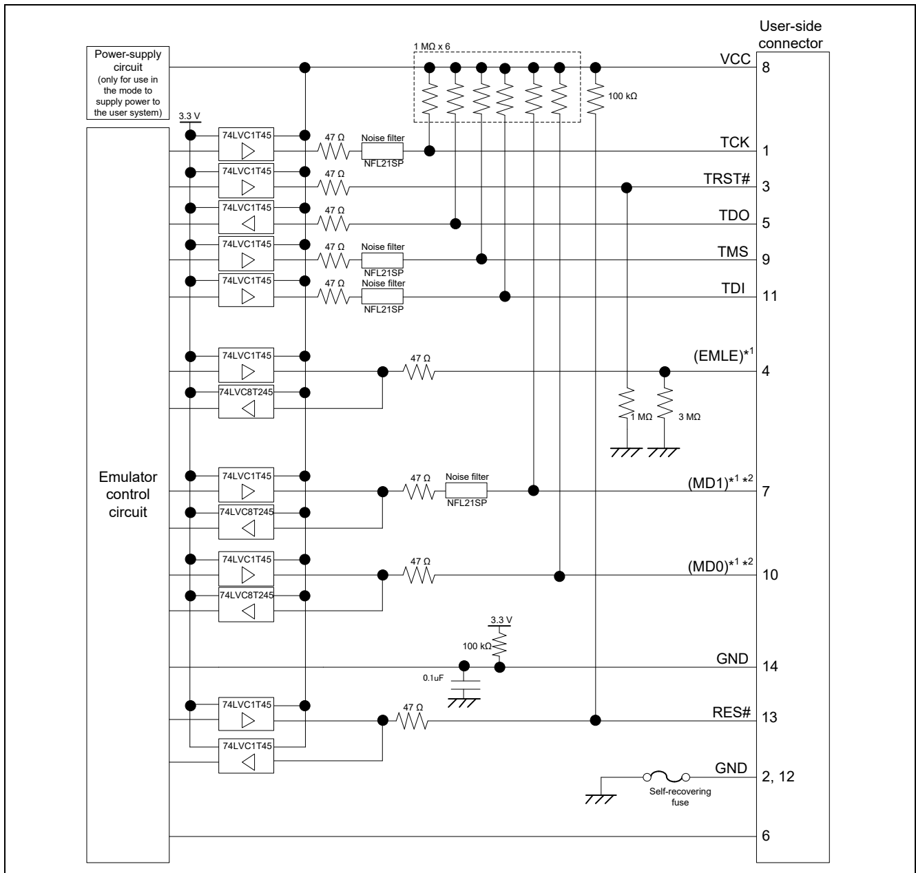
Figure 2.32 Internal Circuits of the E2 with MCUs of the RX600 Series and RX700 Series Connected via the JTAG Interface
