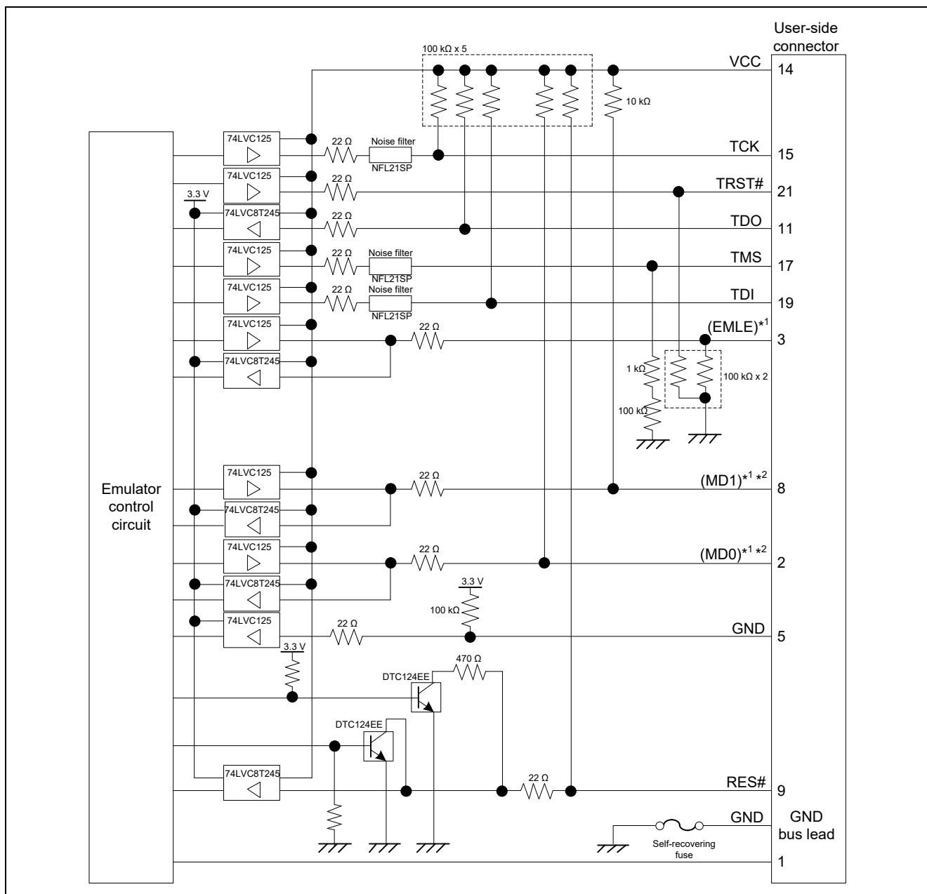
Figure 2.30 Internal Circuits of the E20 with MCUs of the RX600 Series and RX700 Series Connected via the JTAG Interface
