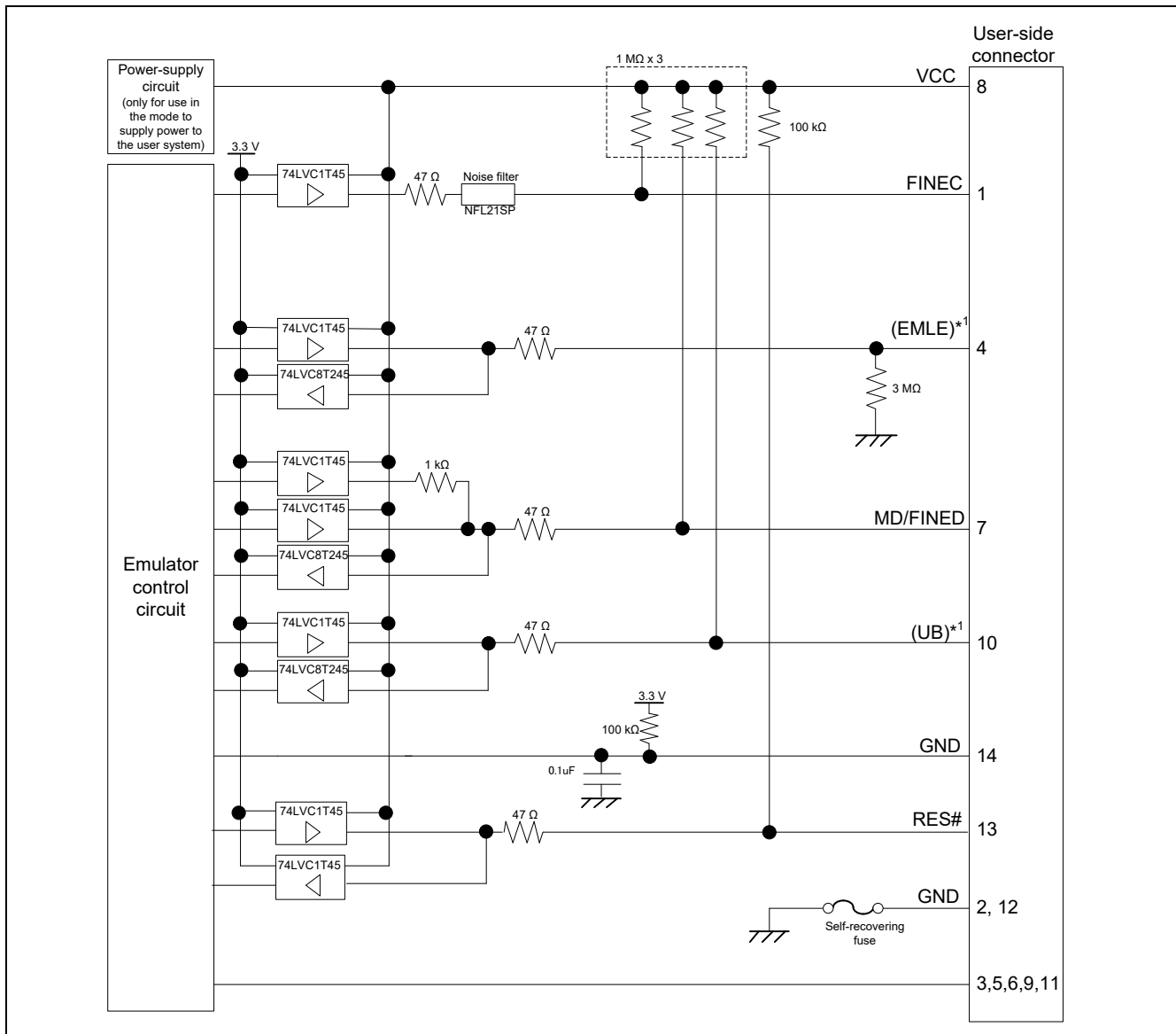
Figure 2.33 Internal Circuits of the E2 with MCUs of the RX63x, RX64x, RX65x, RX66x, RX67x, RX71x, and RX72x Groups Connected via the FINE Interface
