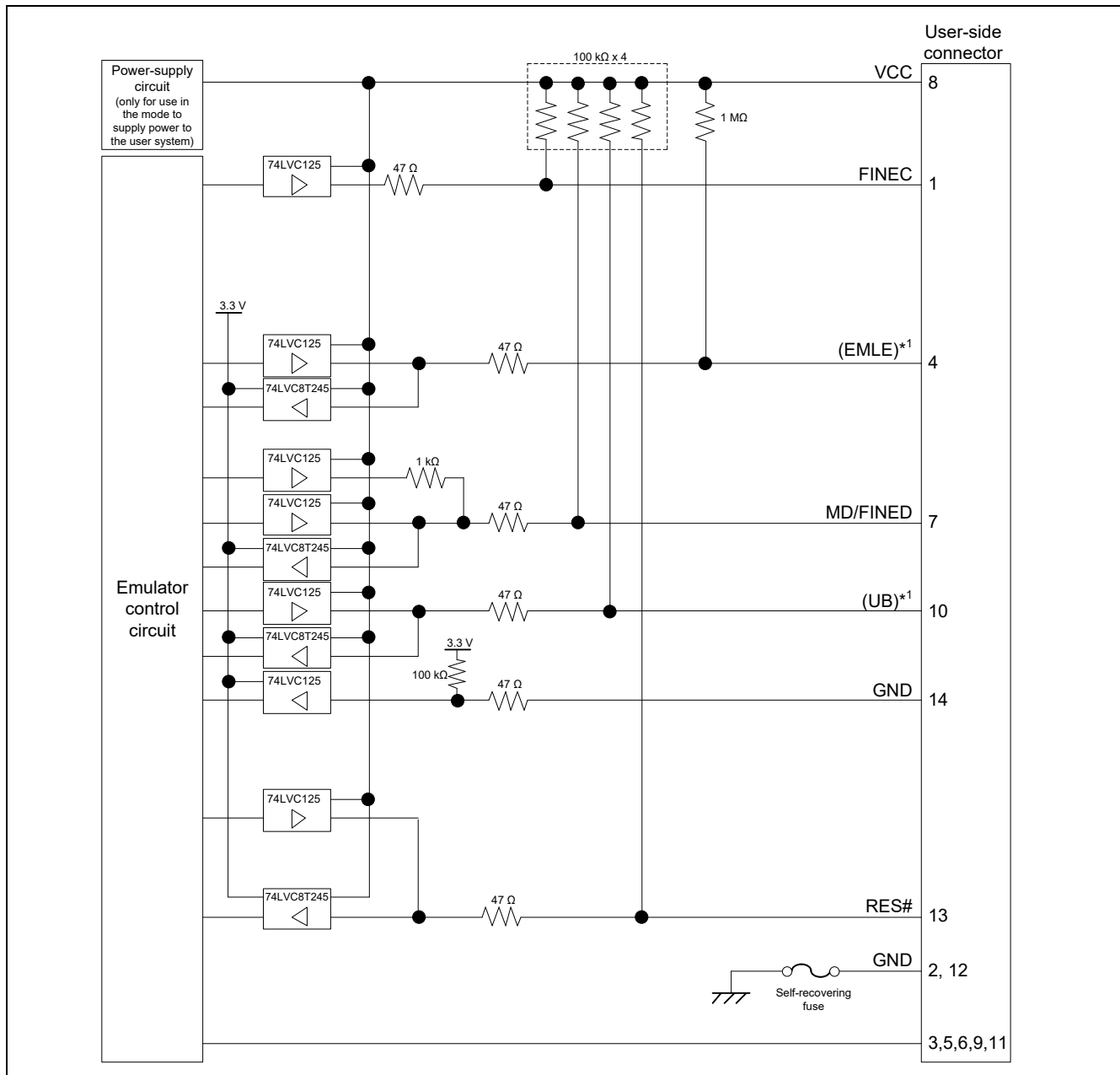
Figure 2.36 Internal Circuits of the E2 Lite with MCUs of the RX63x, RX64x, RX65x, RX66x, RX67x, RX71x, and RX72x Groups Connected via the FINE Interface
