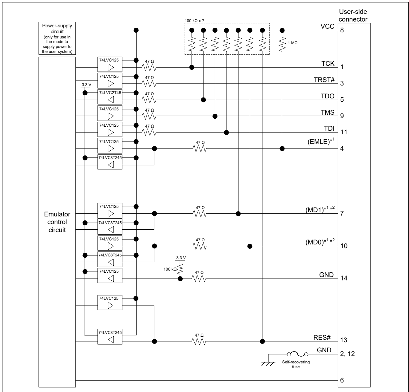
Figure 2.35 Internal Circuits of the E2 Lite with MCUs of the RX600 Series and RX700 Series Connected via the JTAG Interface
