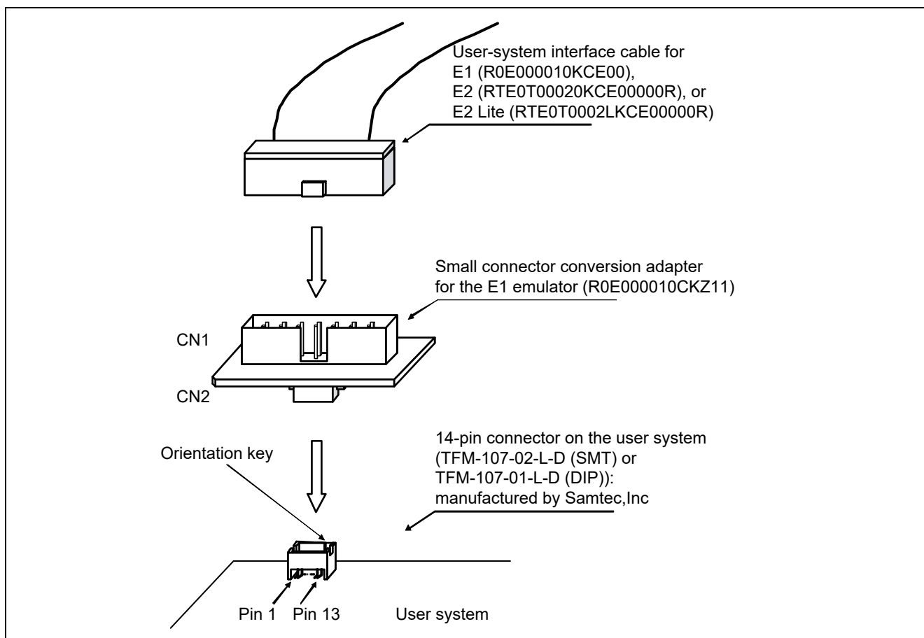
Figure 2.39 Usage of the Small Connector Conversion Adapter for the E1
