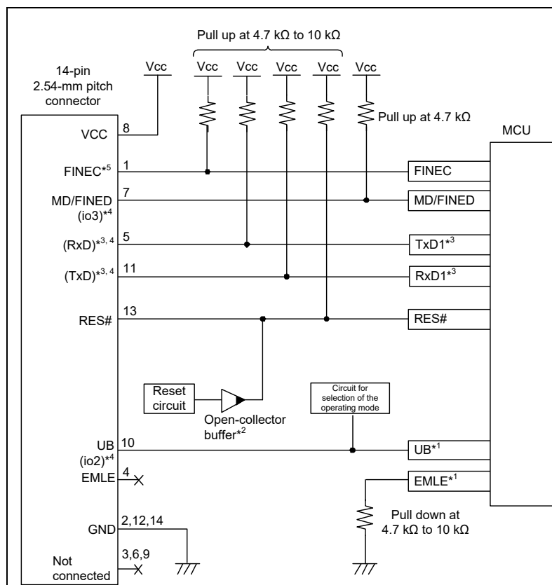
Figure 2.12 Example of Connection between the 14-Pin Connector and MCUs of the RX63x, RX64x, RX65x, RX66x, RX67x, RX71x, and RX72x Groups in FINE Interface Connection (for Debugging and Flash Programming)
