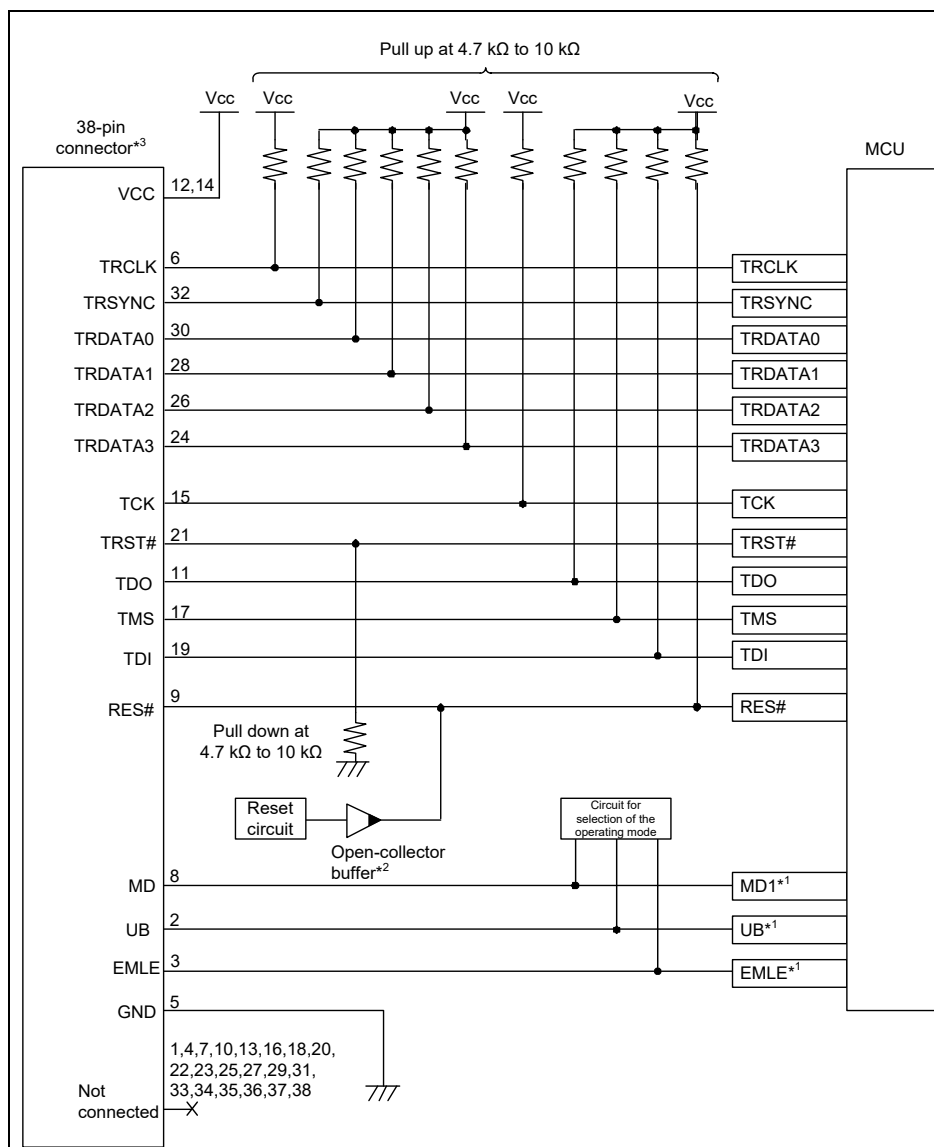
Figure 2.16 Example of Connection between the 38-Pin Connector and MCUs of the RX63x, RX64x, RX65x, RX66x, RX67x, RX71x, and RX72x Groups in JTAG Interface Connection (for Debugging and Flash Programming)
