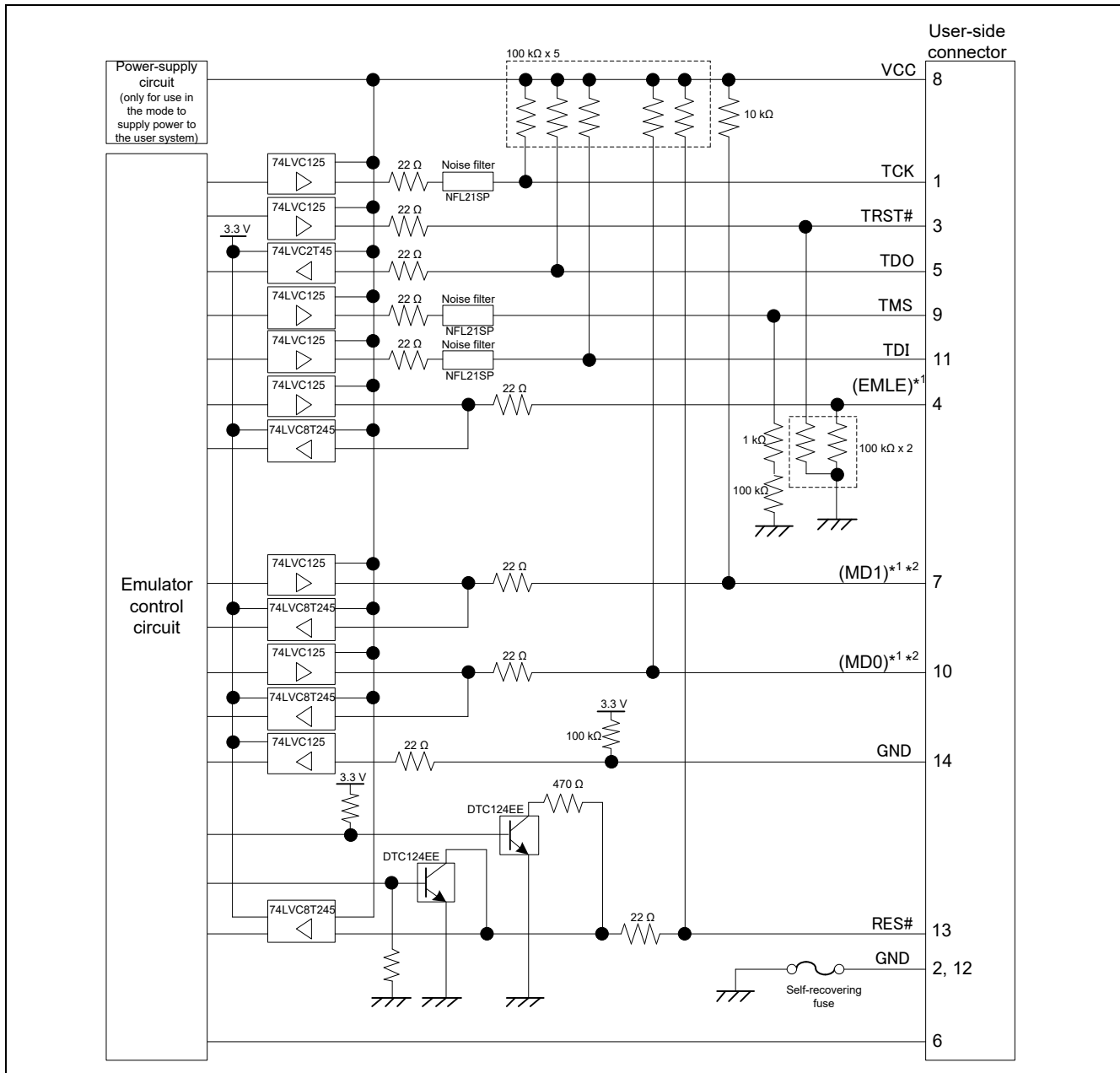
Figure 2.27 Internal Circuits of the E1 with MCUs of the RX600 Series and RX700 Series Connected via the JTAG Interface
