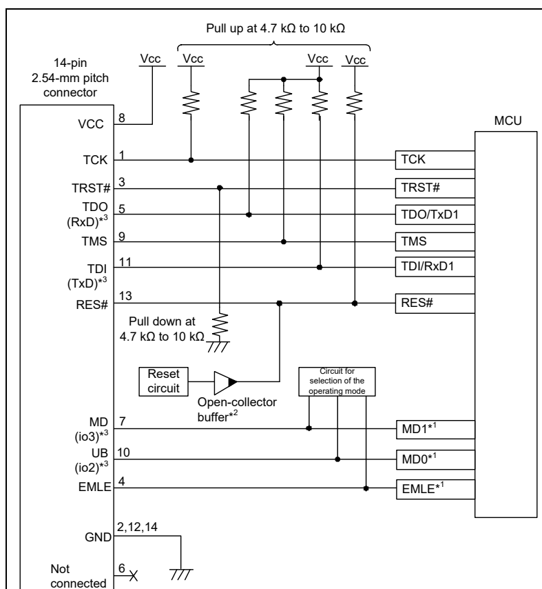
Figure 2.11 Example of Connection between the 14-Pin Connector and MCUs of the RX63x, RX64x, RX65x, RX66x, RX67x, RX71x, and RX72x Groups in JTAG Interface Connection (for Debugging and Flash Programming)
