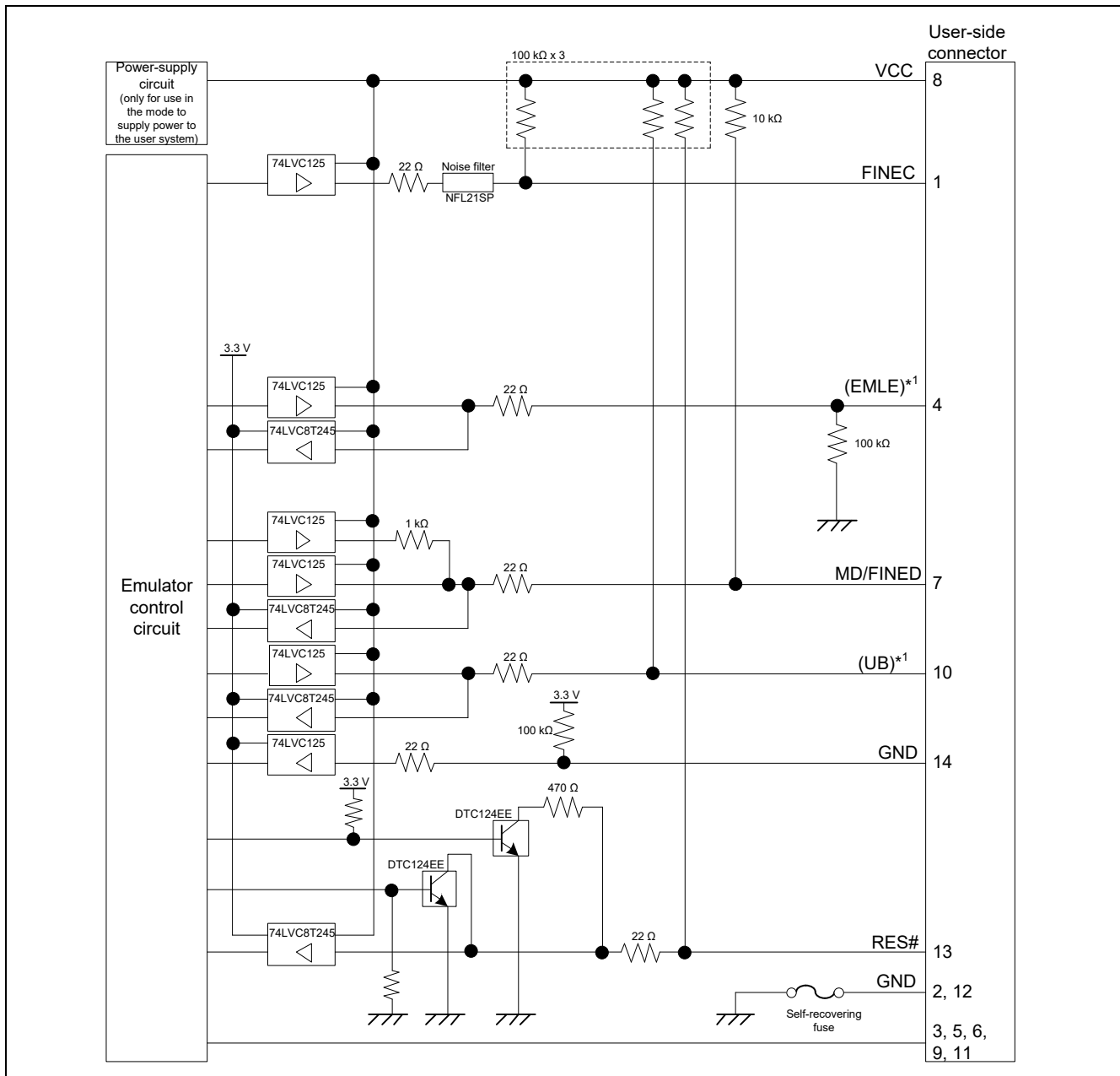
Figure 2.28 Internal Circuits of the E1 with MCUs of the RX63x, RX64x, RX65x, RX66x, RX67x, RX71x, and RX72x Groups Connected via the FINE Interface
