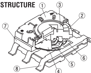
INTERNAL STRUCTURE
