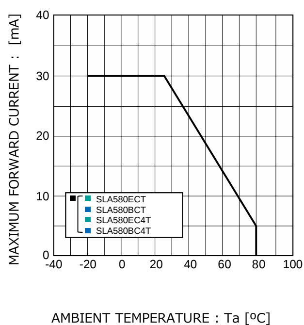
Fig.4 Derating
