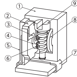
INTERNAL STRUCTURE
