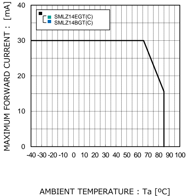
Fig.4 Derating
