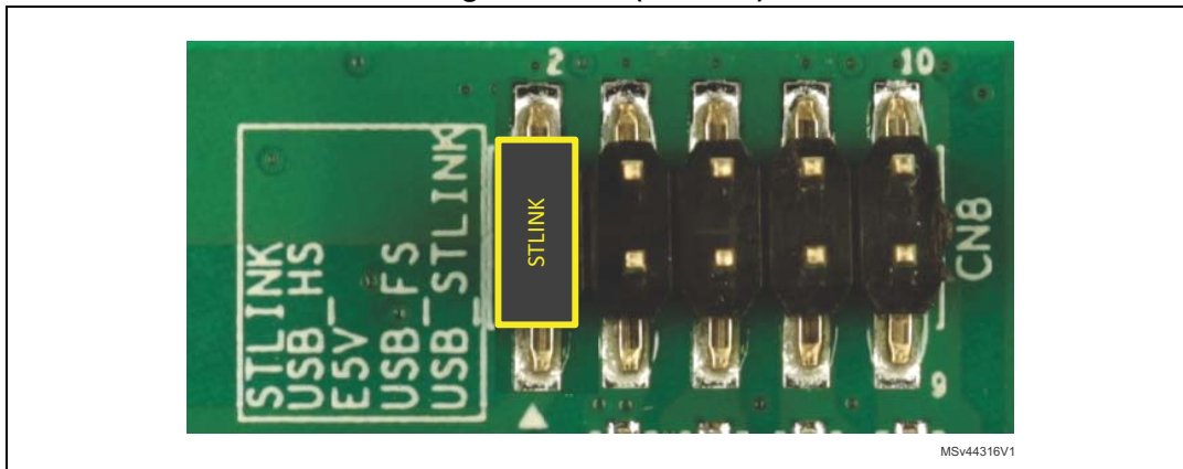
Figure 8. CN8 (ST-LINK)
