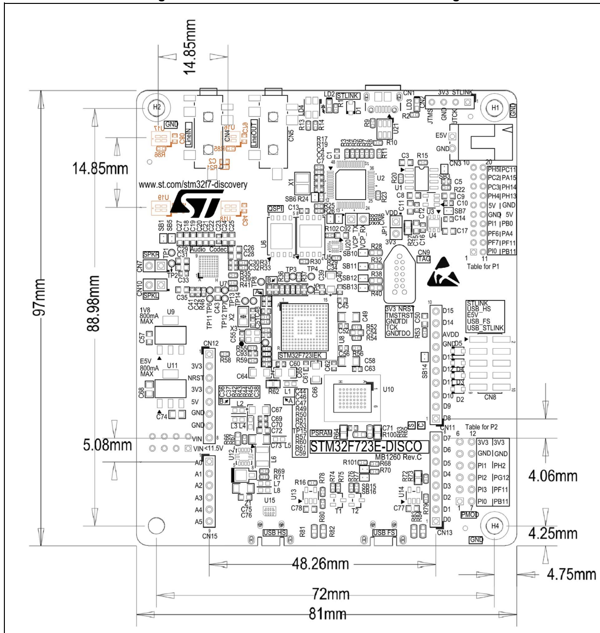
Figure 6. 32F723EDISCOVERY mechanical drawing
