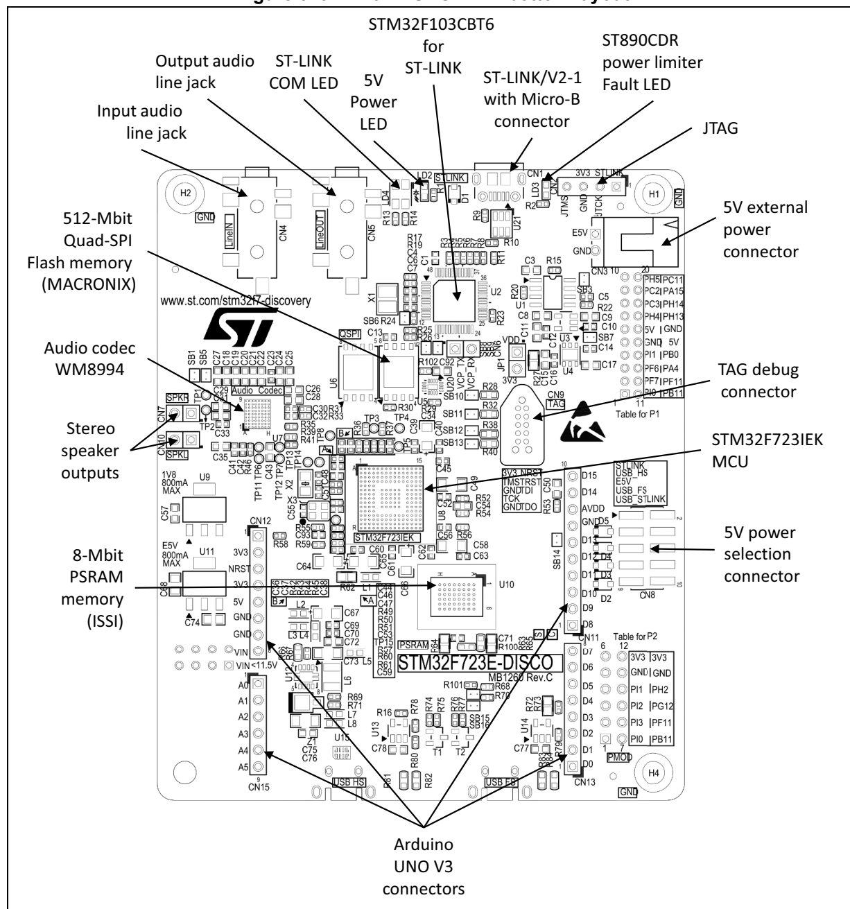
Figure 5. 32F723EDISCOVERY bottom layout
