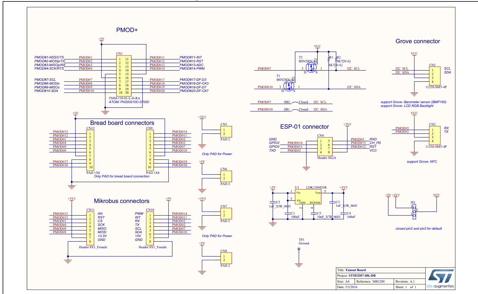
Figure 34. Fanout board
