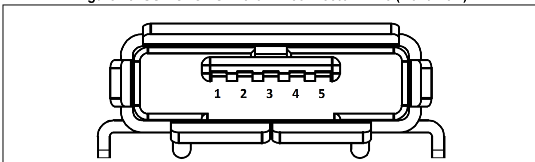
Figure 18. USB OTG FS Micro-AB connector CN18 (front view)
