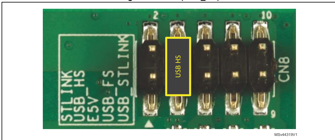
Figure 11. CN8 (USB_HS)
