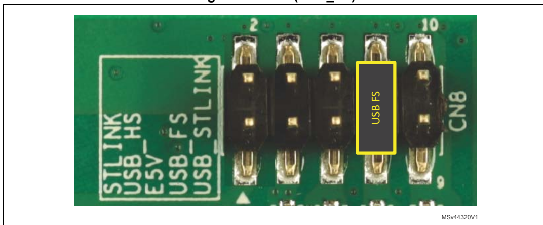
Figure 12. CN8 (USB_FS)
