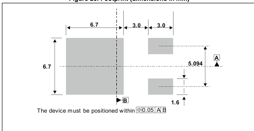
Figure 20. Footprint (dimensions in mm)
