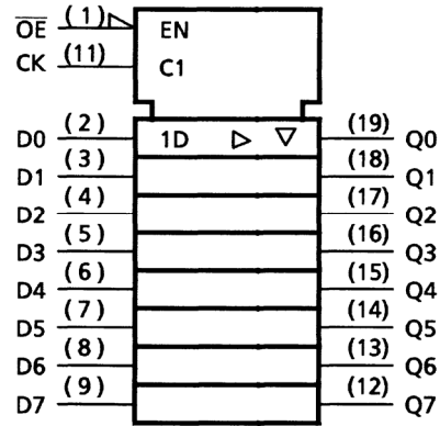
TC74HC574A
