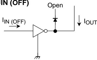
4. I_{IN} (OFF)
