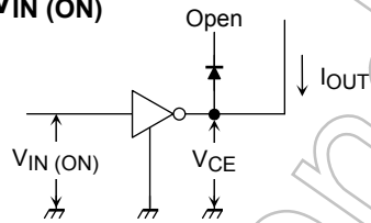
5. V_{IN(ON)}
