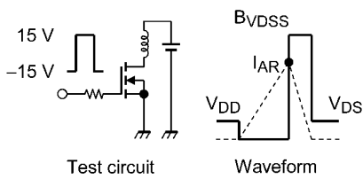
Fig. 8.16 Test Circuit/Waveform
