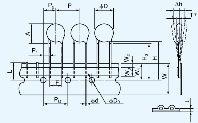
Straight Leads and Taped Z7D □ □ □ T4D
