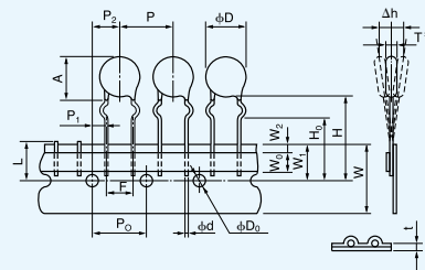
Crimped Leads and Taped Z7D □ □ □ T4C
