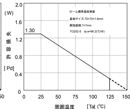
TO252-5
