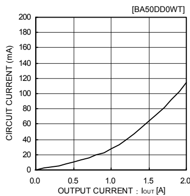
Fig.20 負荷別回路電流 ( I_{out}=0mA \rightarrow 2A )
