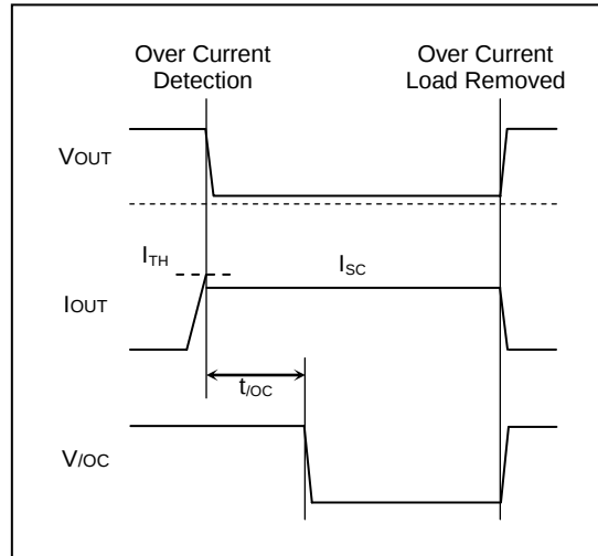
Figure 41. 過電流制限
