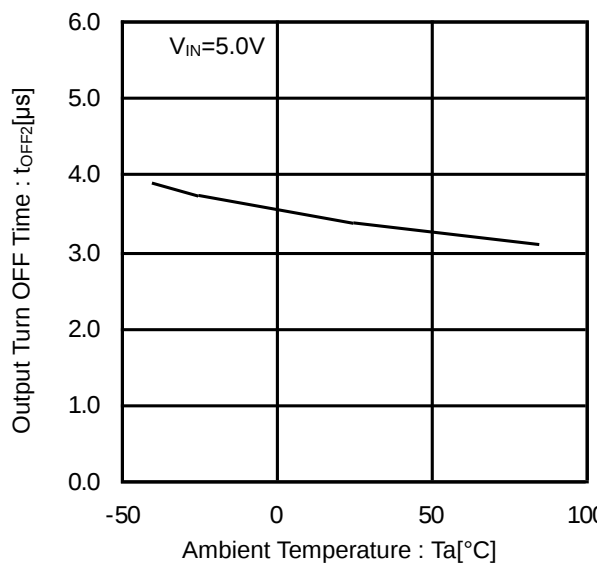
Figure 27. Output Turn OFF Time vs Ambient Temperature
