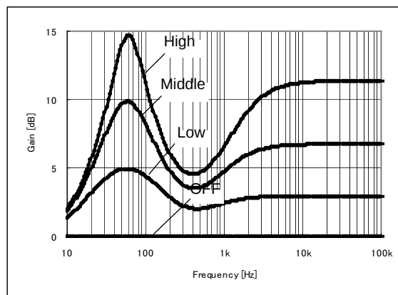
Figure 27. Surround Gain (Surround SW : (B)=ON)の代表特性
