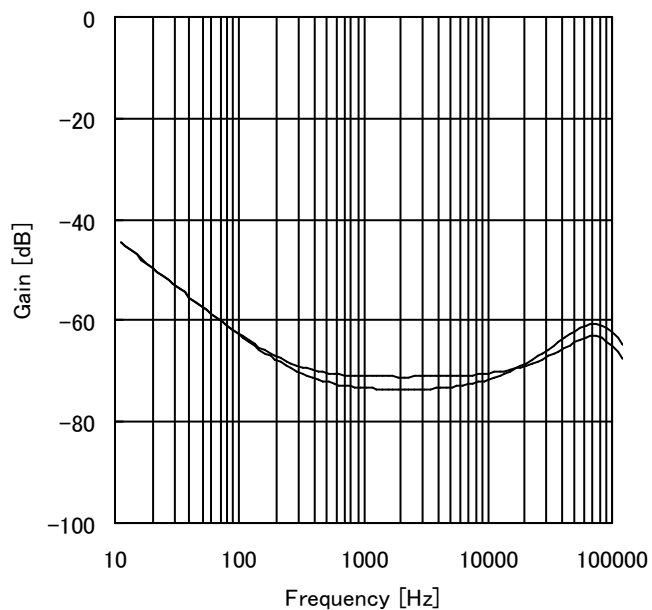
Figure 8. CMRR
