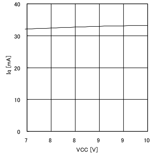
Figure 4. VCCL vs Iq (VCCH=OPEN)
