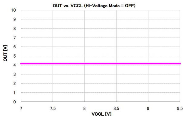
Figure 22. OUT(18～23pin)_DC-Bias = 4.15V fixed. (Hi-Voltage Mode = OFF)
