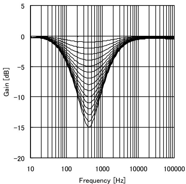
Figure 10. Loudness
