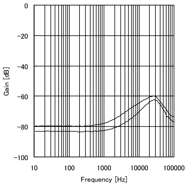
Figure 9. PSRR
