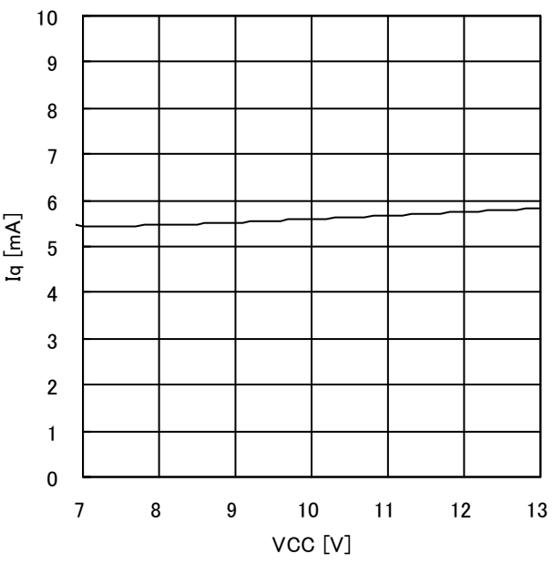
Figure 5. VCCH vs Iq (VCCL=OPEN)
