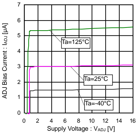
Figure 13. ADJ Bias Current vs Supply Voltage
