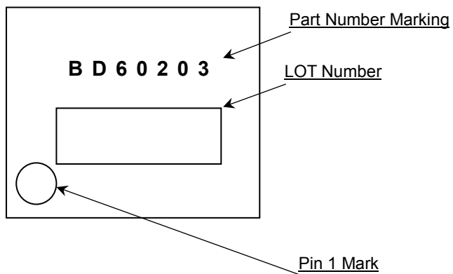
HTSSOP-B24 (TOP VIEW)
