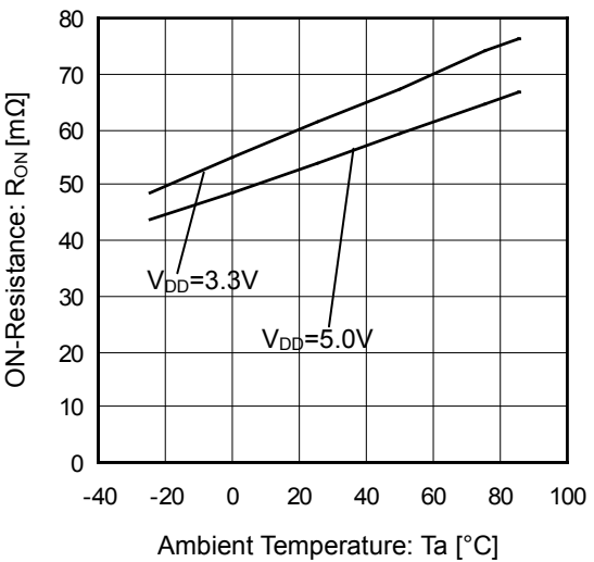
Figure 29. ON-Resistance vs Ambient Temperature
