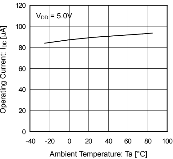
Figure 31. Operating Current vs Ambient Temperature (CTRL Enable)
