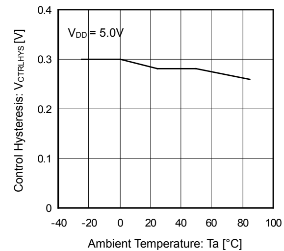
Figure 15. Control Hysteresis Voltage vs Ambient Temperature
