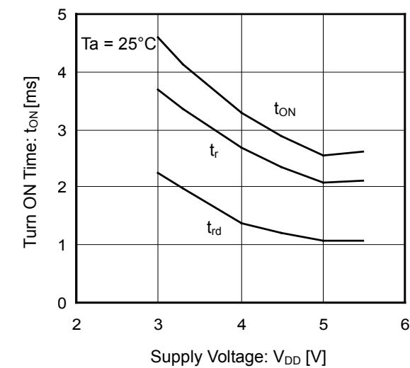
Figure 16. Turn ON Time vs Supply Voltage
