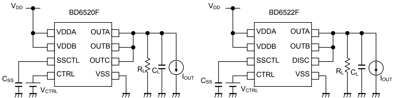
Figure 3. 測定回路
