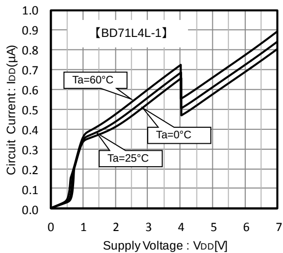
Figure 3. Circuit Current
