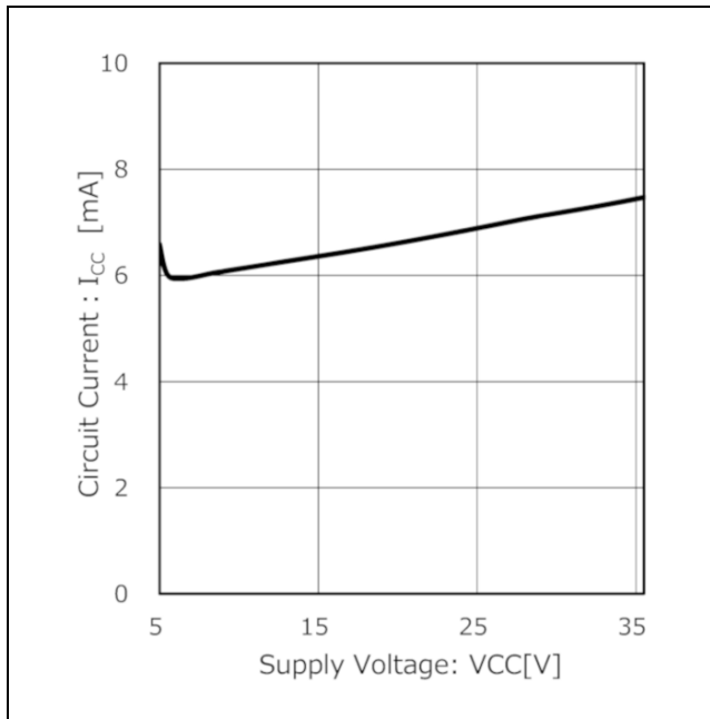
Figure 6. Circuit Current vs Power Supply Voltage ( V_{CC} = 4.5\text{ V} \sim 35\text{ V} , V_{EN} = 3.3\text{ V} , V_{PWM} = 0\text{ V} )
