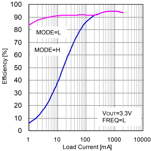
Figure 8. 効率 vs 負荷電流 (VIN=5V, VOUT=3.3V, L=1.0µH, FREQ=L)
