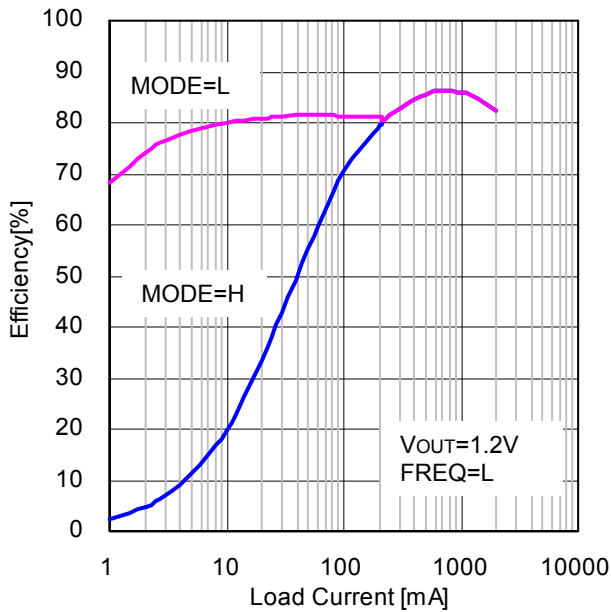
Figure 6. 効率 vs 負荷電流 (VIN=5V, VOUT=1.2V, L=1.0µH, FREQ=L)
