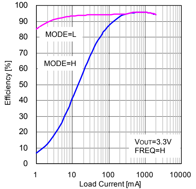
Figure 9. 効率 vs 負荷電流 (VIN=5V, VOUT=3.3V, L=1.5µH, FREQ=H)
