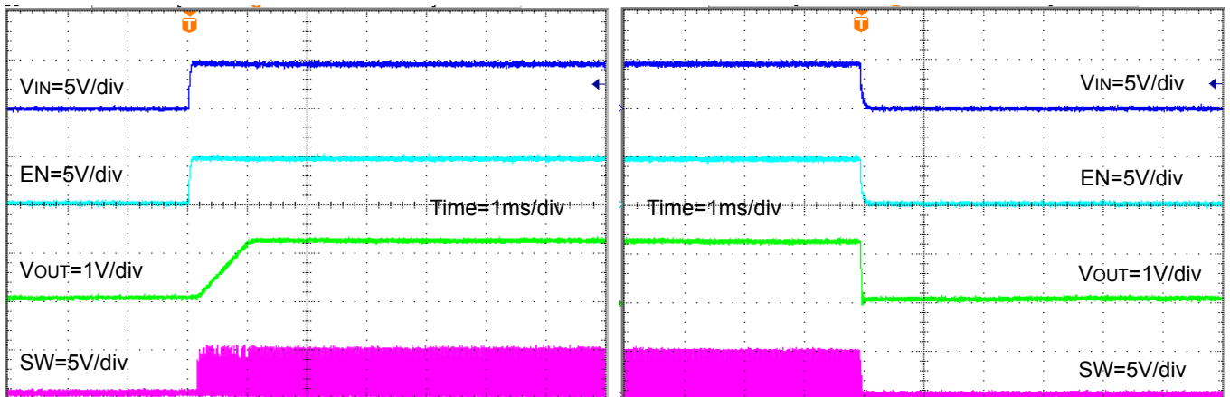
Figure 30. VIN 起動波形 (FREQ=H, RLOAD=0.6Ω)
