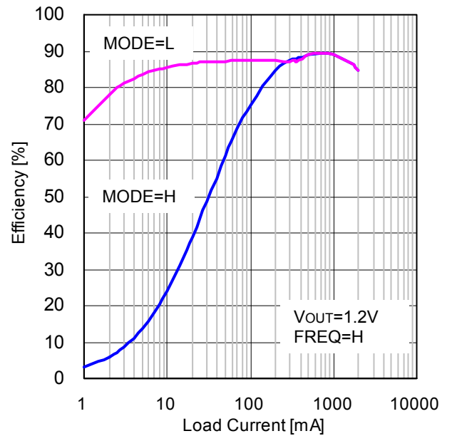
Figure 7. 効率 vs 負荷電流 (VIN=5V, VOUT=1.2V, L=1.5µH, FREQ=H)
