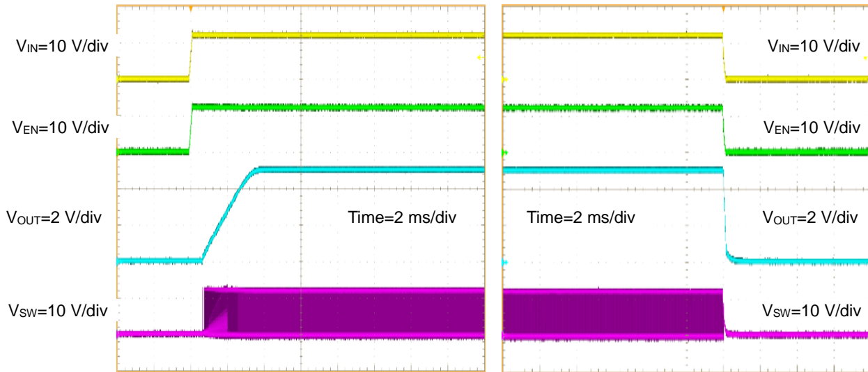
Figure 22. 起動波形 ( V_{IN}=V_{EN} ) I_{OUT}=1.0\text{ A}
