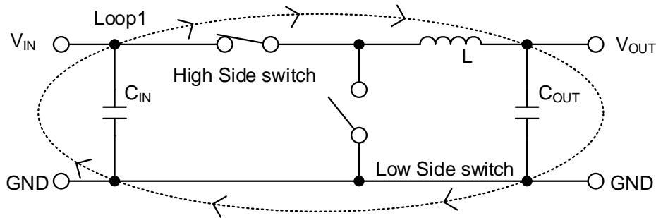
Figure 50-a. High Side switch: ON, Low Side switch: OFF 時の電流経路
