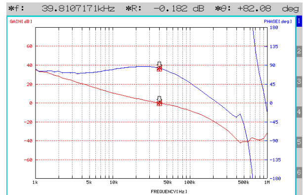
Figure 35. 位相特性 ( V_{IN}=12\text{ V} , V_{OUT}=3.3\text{ V} , I_{OUT}=1\text{ A} , C_{OUT}=\text{Ceramic}10\ \mu\text{Fx}3 )
