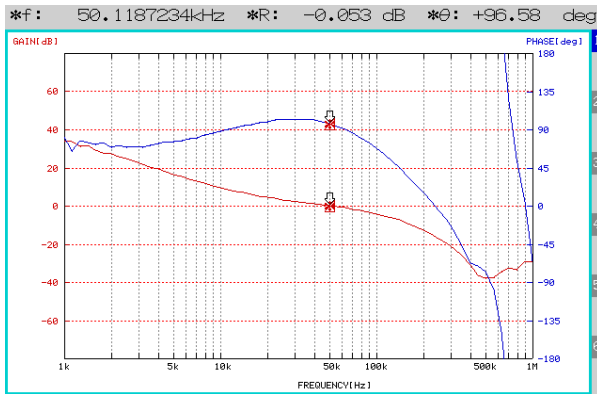
Figure 34. 位相特性 ( V_{IN}=12\text{ V} , V_{OUT}=5\text{ V} , I_{OUT}=1\text{ A} , C_{OUT}=\text{Ceramic}10\ \mu\text{Fx}3 )
