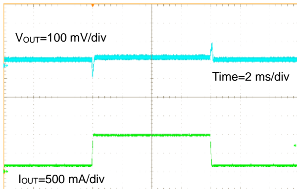
Figure 36. 負荷応答波形 I_{OUT}=0.2\text{ A} - 1\text{ A} ( V_{IN}=12\text{ V} , V_{OUT}=5\text{ V} , C_{OUT}=\text{Ceramic}10\ \mu\text{Fx}3 )
