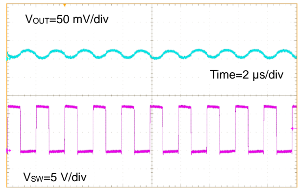
Figure 40. PWM 制御時 SW 波形 (V IN = 12 V, V OUT =5.0 V, I OUT =1 A)
