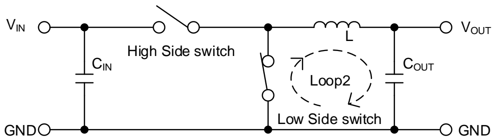
Figure 50-b. High Side switch: OFF, Low Side switch: ON 時の電流経路
