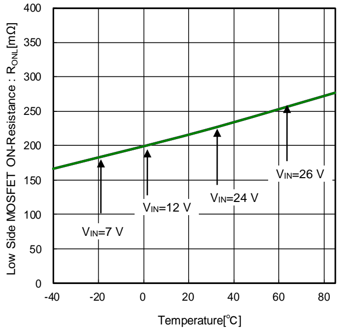
Figure 11. 下側 MOSFET ON 抵抗 vs 周囲温度
