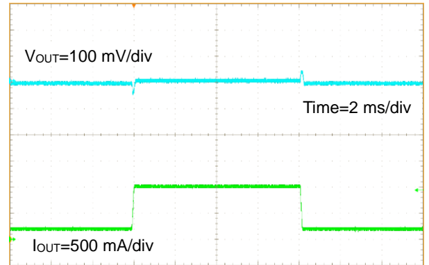
Figure 37. 負荷応答波形 I_{OUT}=0.2\text{ A} - 1\text{ A} ( V_{IN}=12\text{ V} , V_{OUT}=3.3\text{ V} , C_{OUT}=\text{Ceramic}10\ \mu\text{Fx}3 )
