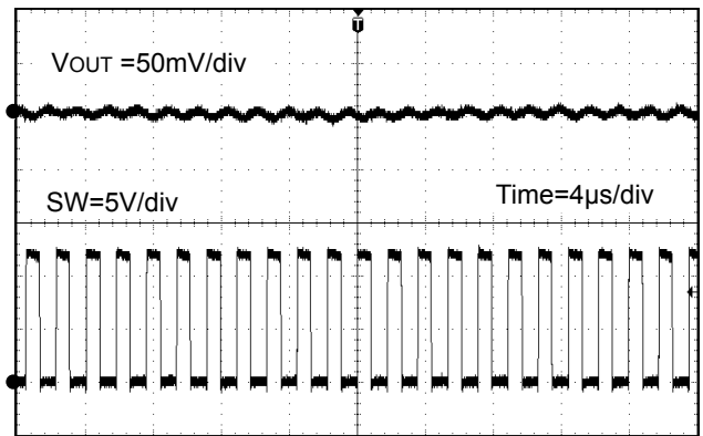
Figure 34. スイッチング波形(②PWM control) (VIN = 12V, VOUT = 5.0V, IOUT = 3A)
