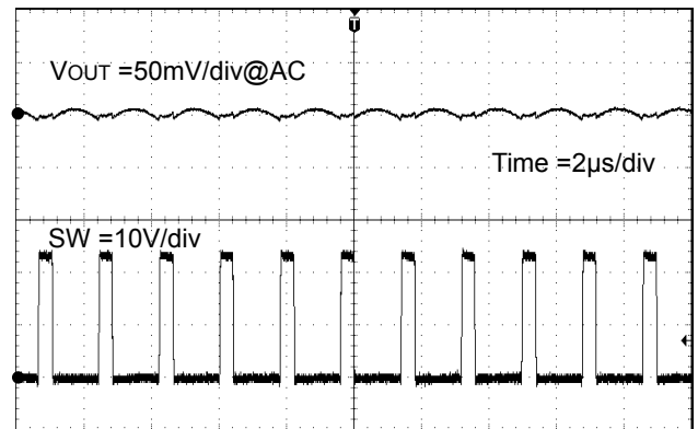
Figure 42. V_{OUT} リップル波形 ( V_{IN} = 24V , V_{OUT} = 5V , R_3=10k\Omega )
