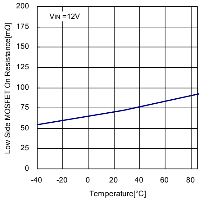
Figure 11. 下側 MOSFET ON 抵抗 vs 周囲温度
