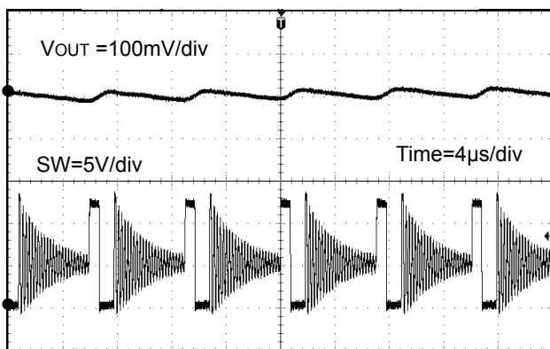
Figure 33. スイッチング波形(①SLLM™ control) (VIN = 12V, VOUT = 5.0V, IOUT = 50mA)
