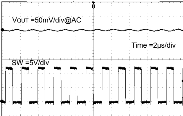
Figure 41. V_{OUT} リップル波形 ( V_{IN} = 12V , V_{OUT} = 5V , R_3=10k\Omega )
