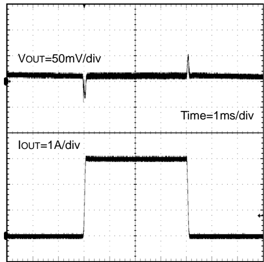
Figure 40. 負荷応答波形 IOUT=0A - 3A (VIN=5V, VOUT=1.8V, COUT=Ceramic 44μF)
