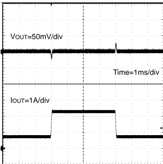
Figure 39. 負荷応答波形 IOUT=0.75A - 2.25A (VIN=5V, VOUT=1.8V, COUT=Ceramic 44μF)
