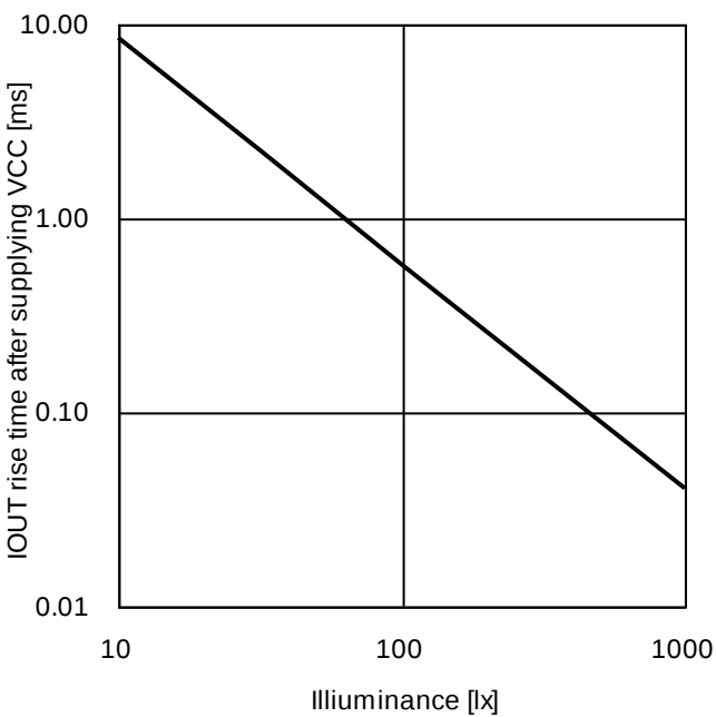
Figure 4. IOU_T rise time after supplying VCC vs Illuminance
