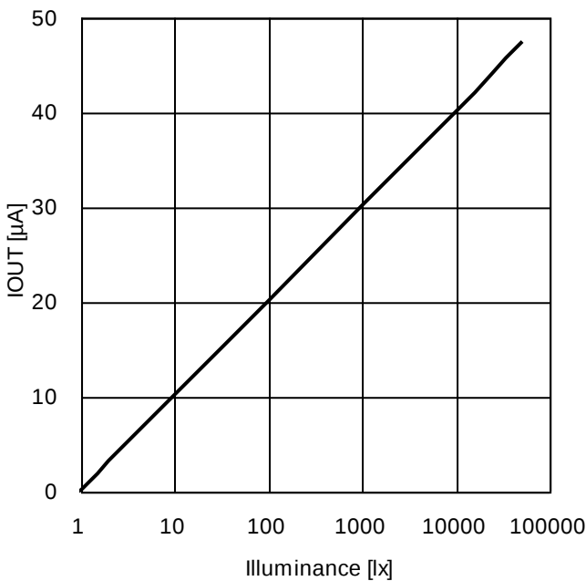
Figure 2. IOU_T vs Illuminance
