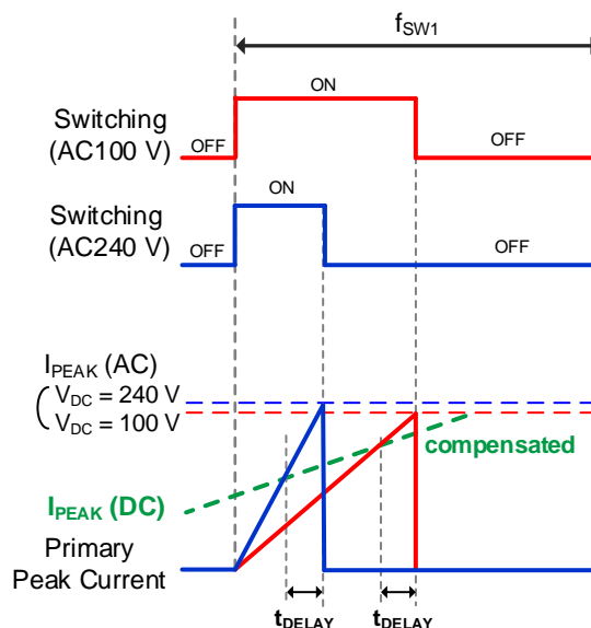
Figure 9. With the AC Voltage Compensation Function
