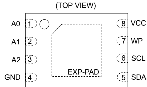
Figure 3-(b). 端子配置図 (VSON008X2030 *1 、VSN08AX2030A) *1 Last Time Buy.
