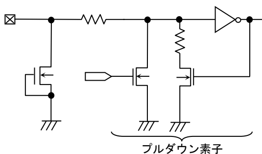
Figure 58. 入力端子回路図 (A1, A2, WP)
