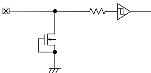
Figure 59. 入力端子回路図 (SCL)
