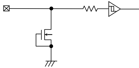
Figure 60. 入力端子回路図 (SCL)
