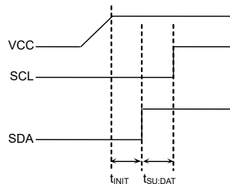
Figure 58. SCL='LOW' SDA='LOW'の時
