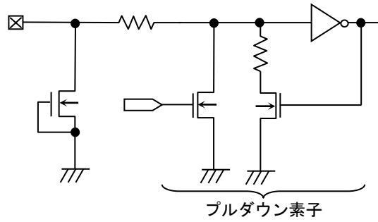
Figure 59. 入力端子回路図 (A0, A1, A2, WP)
