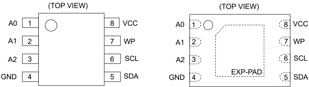
Figure 3-(a). 端子配置図 (SOP8*1、SOP-J8、TSSOP-B8、MSOP8) *1 Last Time Buy. Figure 3-(b). 端子配置図 (VSON008X2030*1、VSON08AX2030)
