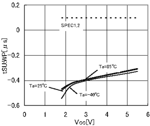
Figure 32. WP setup time t_{SU:WP}
