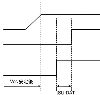
Figure 61. SCL='L' SDA='L'の時
