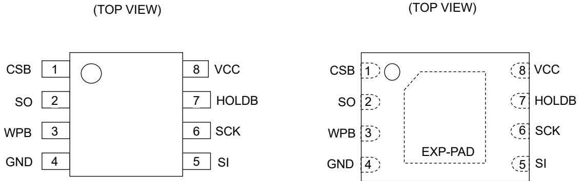
Figure 3-(a). 端子配置図 (SOP8*1、SOP-J8、TSSOP-B8、MSOP8) *1 Last Time Buy.
